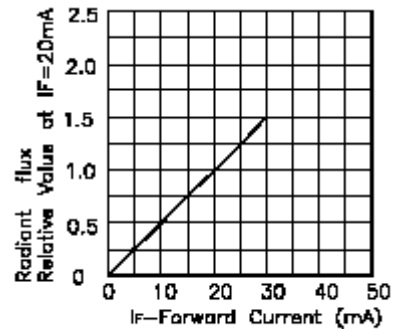
RADIANT FLUX Vs. FORWARD CURRENT
